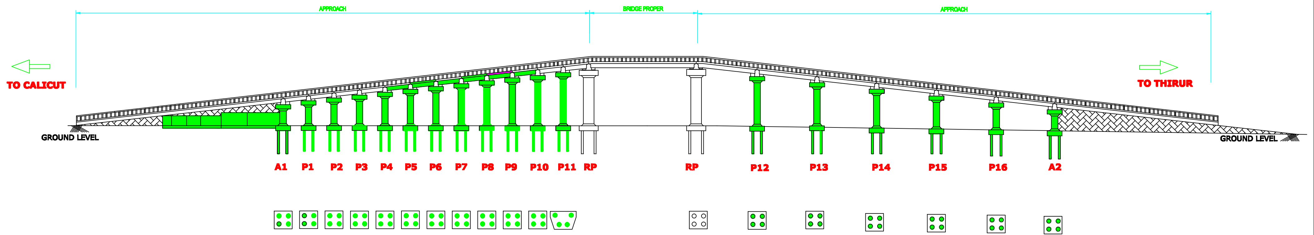
PILE FOUNDATION
